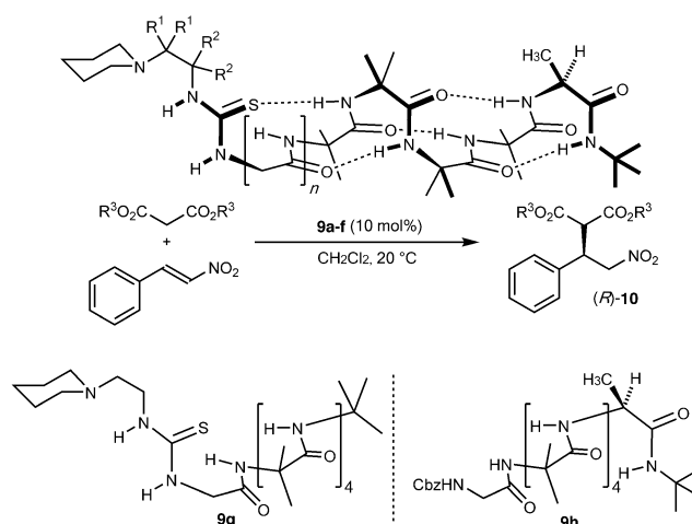
Figure 3. Catalytic foldamers with a remotely inducible catalytic site.
